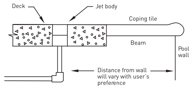
Drawing shows simplicity of installation—similar to other pool plumbing tasks.
