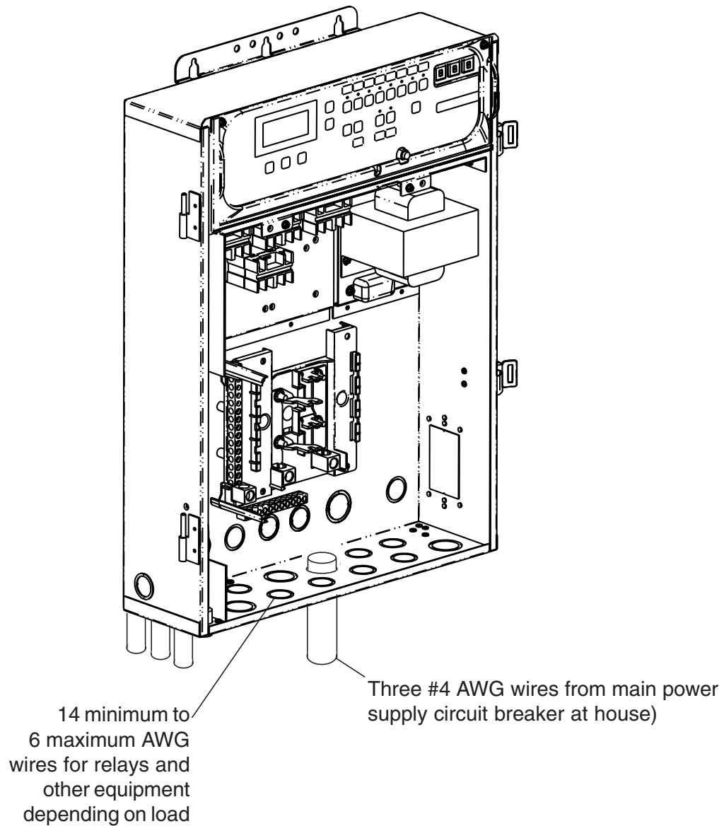
EasyTouch Load Center (front view) with front door and high voltage panel removed
