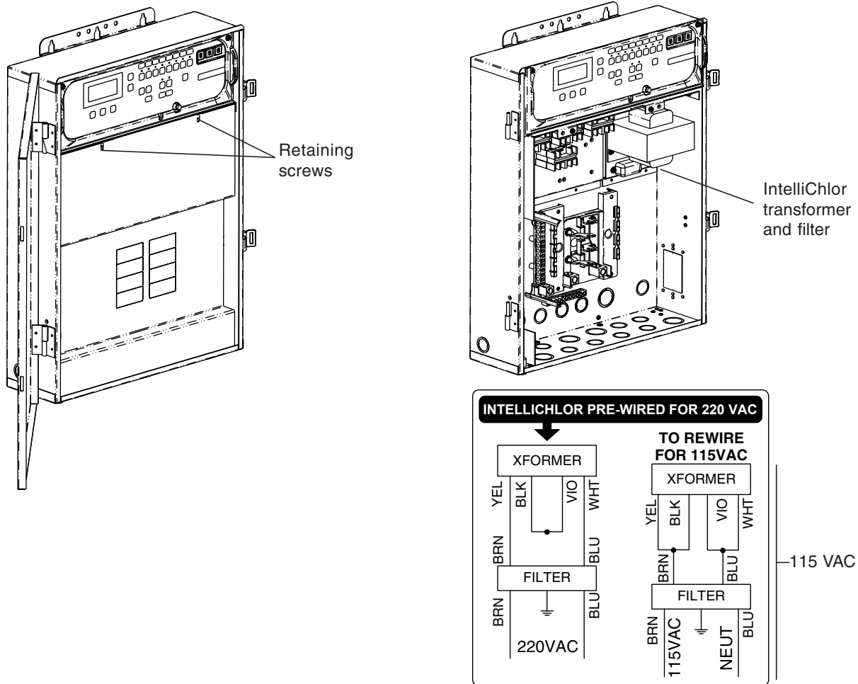
IntelliChlor transformer and filter wiring diagram
