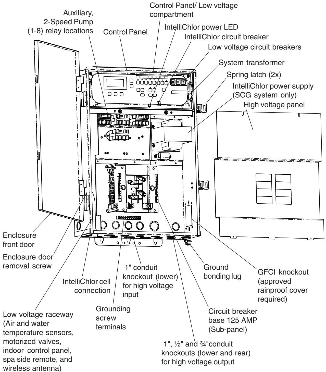
EasyTouch Load Center (23" H x 17" W x 4 3/4" D)
