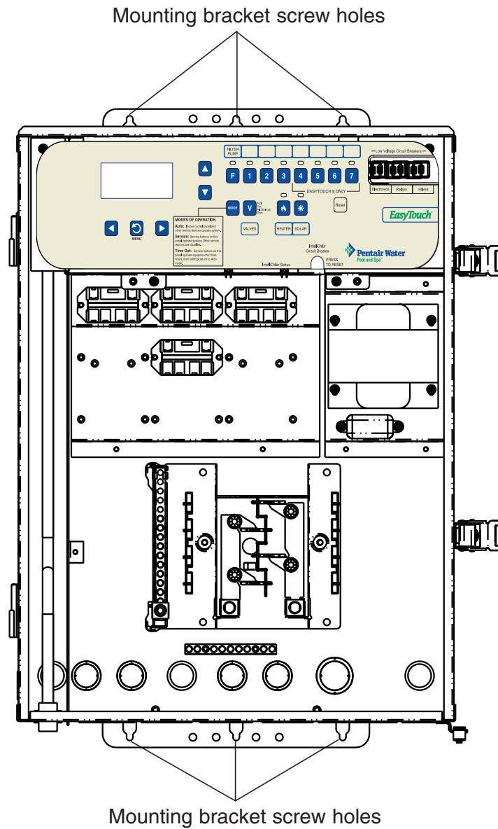
EasyTouch Load Center (front view) with front door and high voltage panel removed
