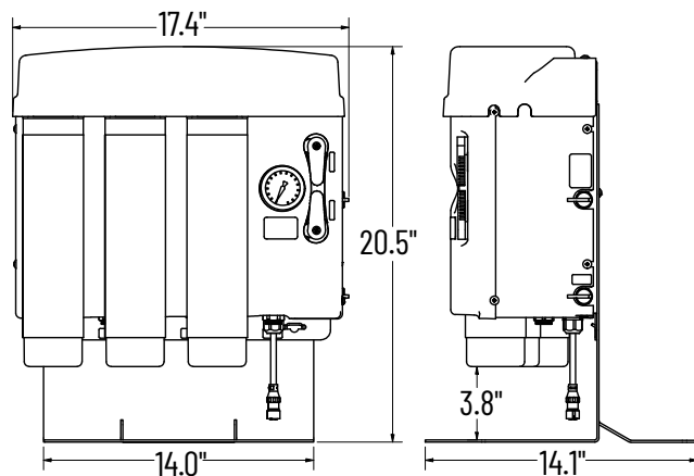
Processor with Size 4 Cannisters on Optional Stand
