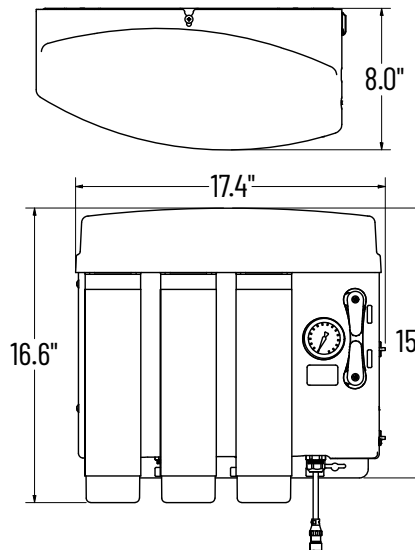
Processor with Size 4 Cannisters, Wall Mounted
