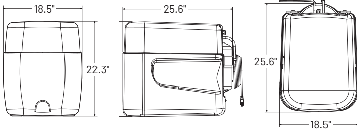
16-gallon atmospheric tank
